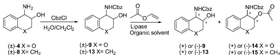
Scheme 4. Enzymatic acetylation of N -protected 1,2-amino alcohols (±)- cis - and (±)- trans -9 and -13 employing vinyl acetate and lipases.
