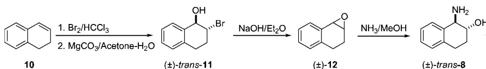
Scheme 3. Chemical procedure for the preparation of (±)-trans-1-amino-1,2,3,4-tetrahydronaphthalen-2-ol [(±)-trans-8].
