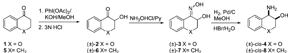
Scheme 1. Chemical synthesis of (±)-cis-4 and (±)-cis-8.
