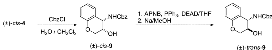
Scheme 2. Synthesis of (±)-trans-4-(benzyloxycarbonylamino)chroman-3-ol [(±)-trans-9].
